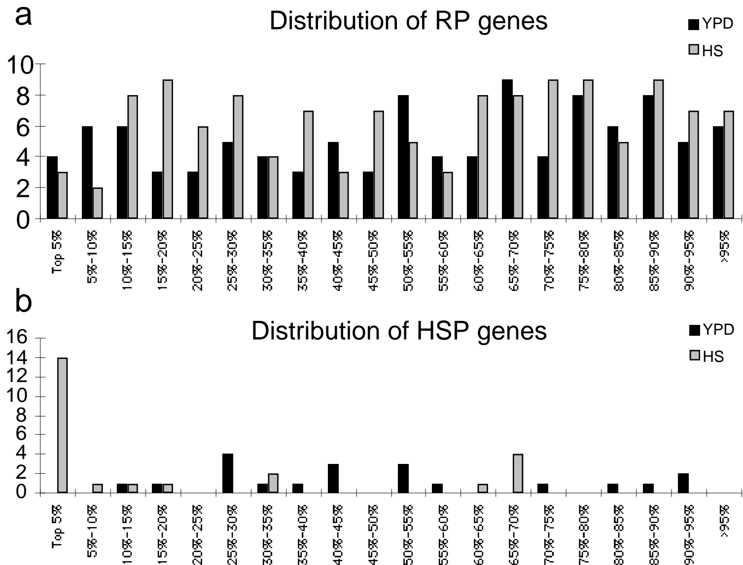
Figure S2 Mediator preferentially associates with heat shock response genes upon heat shock. (a) Distribution of ribosomal protein promoters when promoters were ordered by their P values. (b) Distribution of heat shock response genes when promoters were ordered by their P values.
